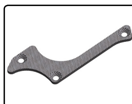
C-00180-273 Suspension arm stiffener - A - Lower Front - Left - Graphite 1.5mm - 1 pc
